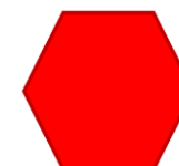
hexagon
